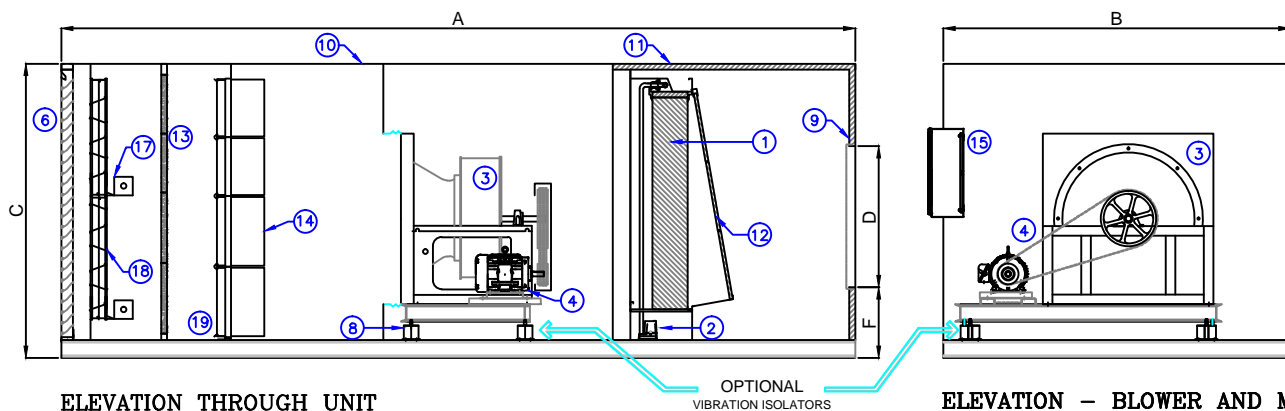
ELEVATION THROUGH UNIT
