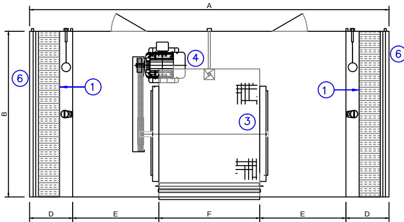
INTERNAL PLAN VIEW
