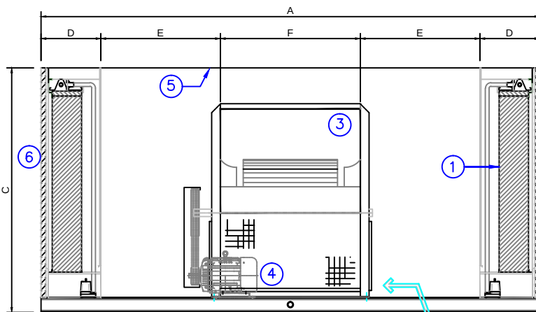
FRONT ELEVATION
